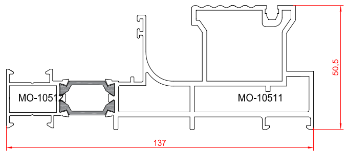
sliding fix frame 2.525 kg/m
