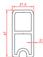
balancer 1.054 kg/m
