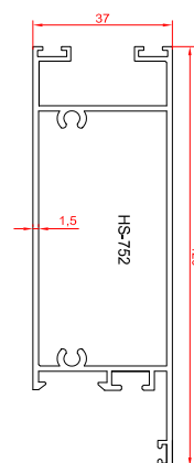
profile for bottom of door
