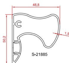
handle 0.907 kg/m
