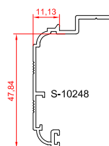
border profile
