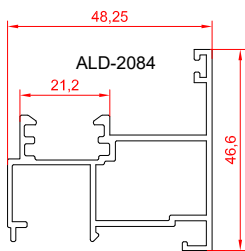
the middle vent profile
