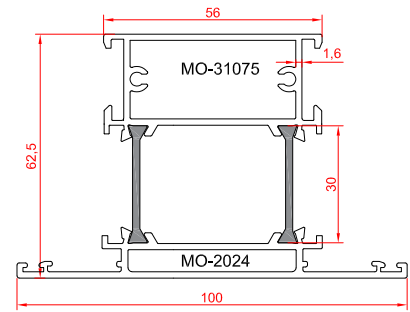
T PROFILE 2.100 kg/m
