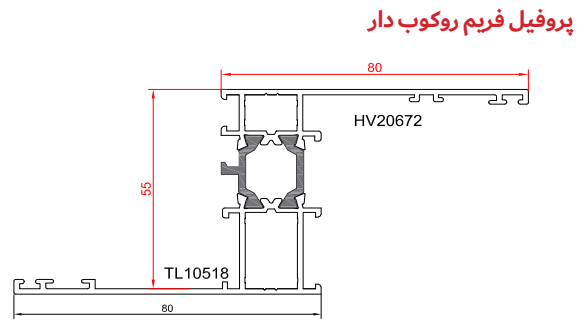
frame profile 1,589 kg/m
