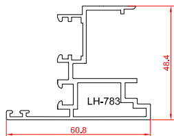
the middle vent profile
