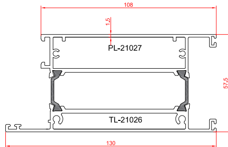
profile for bottom of door 2.608 kg/m
