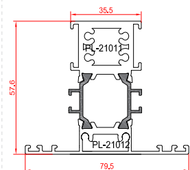
tripetalous profile 2.193 kg/m
