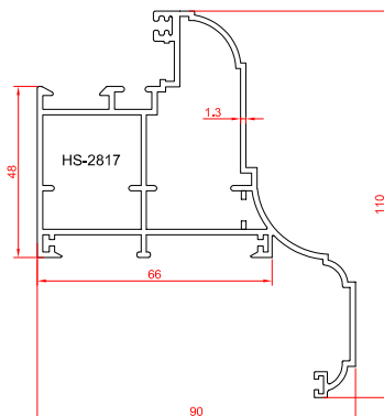
frame profile
