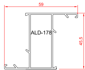
vent profile
