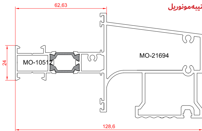
corner profile 2.661 kg/m
