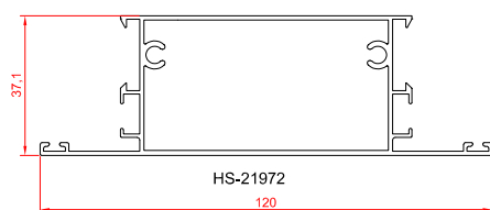
T profile
