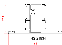
T profile
