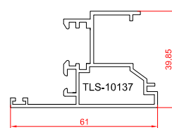
the middle vent profile
