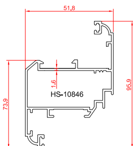
vent profile
