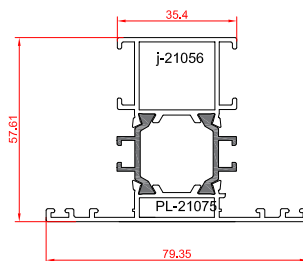
pivot opening adapter 1.451 kg/m
