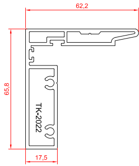
adapter profile 1.624 kg/m
