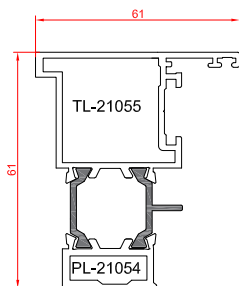
pivot opening adapter 1.549 kg/m
