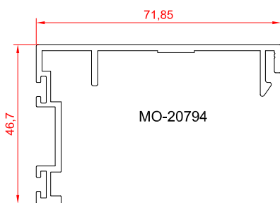
cap for vent 0.701 kg/m
