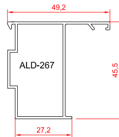
axial opening profile
