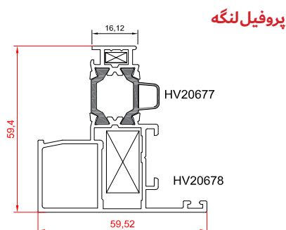
vent profile 1,32 kg/m
