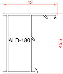
frame profile
