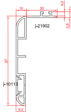
border profile 87 mm 0.846 kg/m
