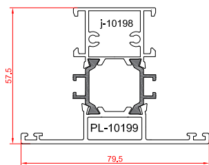
tripetalous profile 1.499 kg/m
