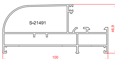
three rail engraving profile
