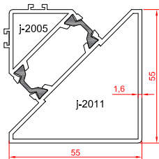
corner profile
