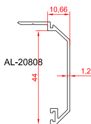
border profile
