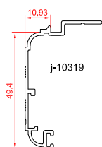
border profile 0.422 kg/m
