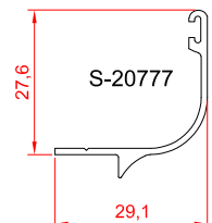
gride rail profile 0.234 kg/m
