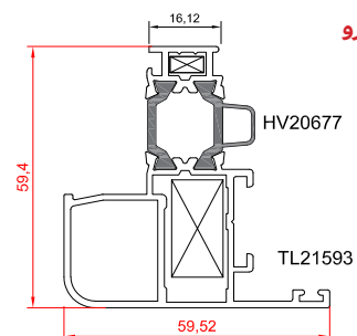
curve profile 1,339 kg/m
