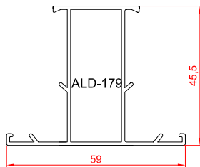
tripetalous profile
