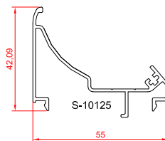
rotating frame profile
