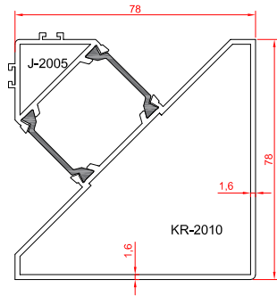
corner profile
