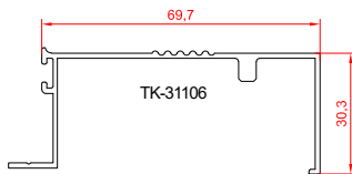
cover frame 0.573 kg/m
