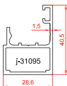
glass support
