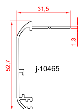
border profile
