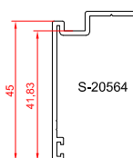
border profile
