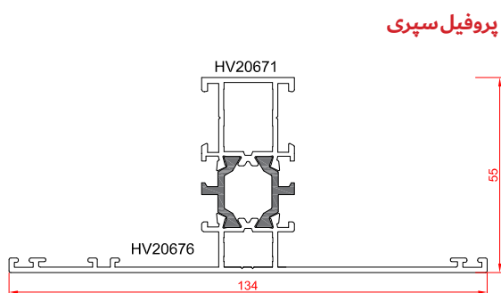
tripetalous profile 1,84 kg/m
