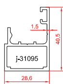
glass support
