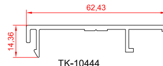
cap for three sash sliding 0.432 kg/m
