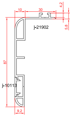
border profile 87 mm
