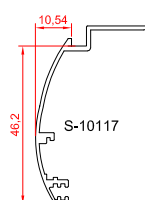
border profile
