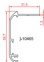
border profile 0.398kg/m
