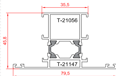
tripetalous profile 1.282 kg/m
