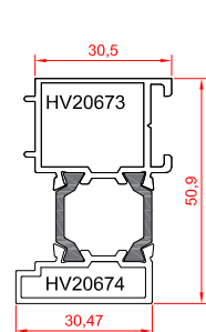
adapter profile 1,047 kg/m
