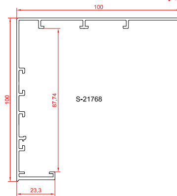
border profile 10*10 cm 1.173 kg/m
