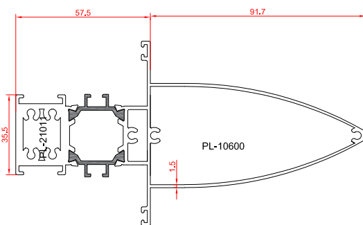
tripetalous profile 2.849 kg/m
