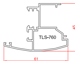
the middle vent profile
