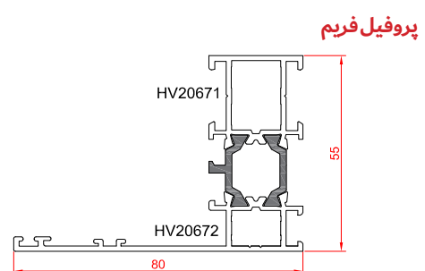
frame profile 1,44 kg/m
