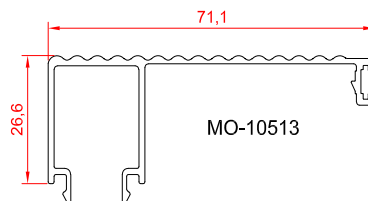
corner profile 0.603 kg/m
