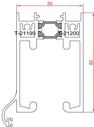
cornice profile 2.820 kg/m
