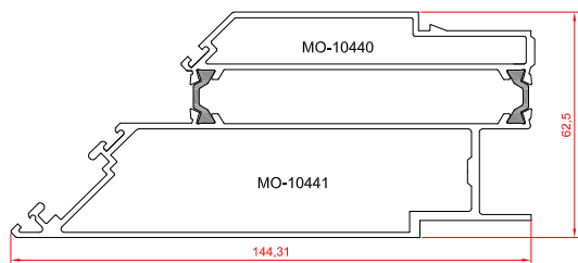
corner profile 3.301 kg/m
