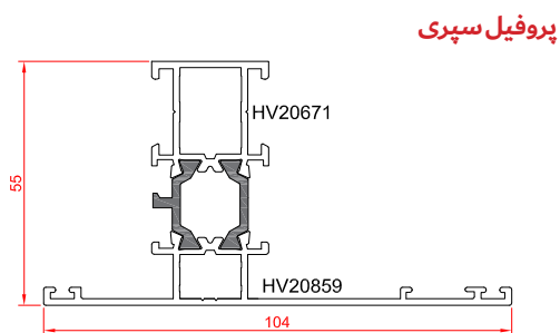
tripetalouse profile 1,411 kg/m
