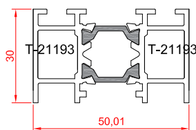
vertical frame profile 1.098 kg/m
