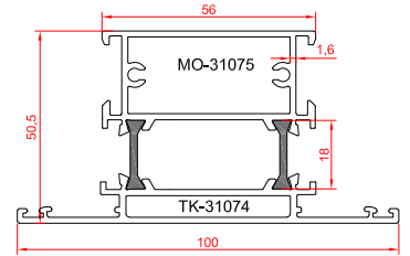
tripetalous profile
