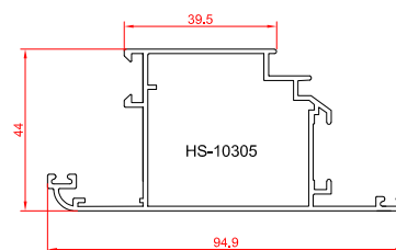
outer opening door profile
