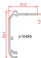
border profile
